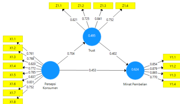
Figure 2. Partial Least Square (PLS) Schematic
