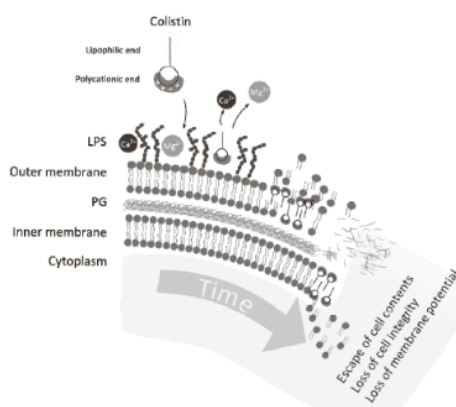
Figure 4. Mechanism of action of colistin 1
