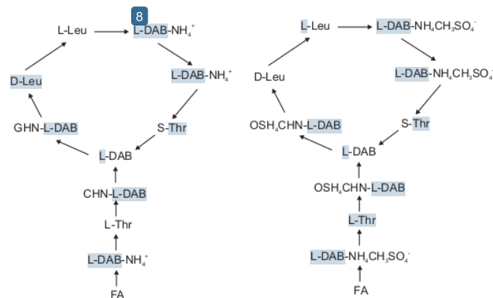
Figure 3. Chemical structure of colistin (left) and colistimethate sodium (right) 1
