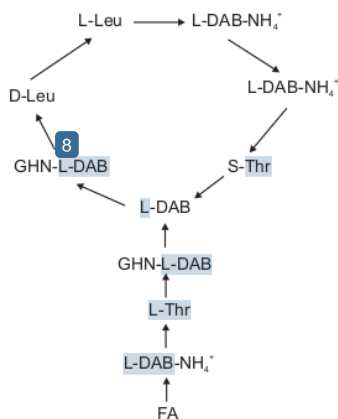
Figure 1. Chemical structure of Colistin 1
