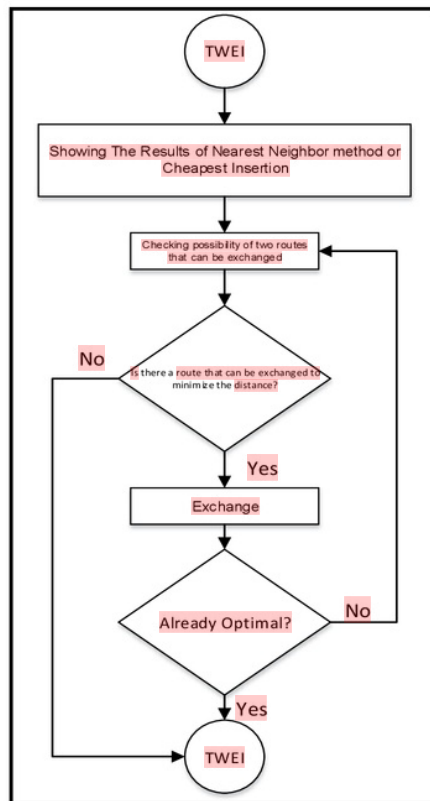
Figure 5. Two-Way Exchange improvement used in WinQSB
