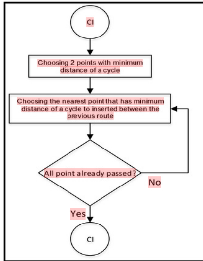
Figure 4. Cheapest Insertion Algorithm used in WinQSB
