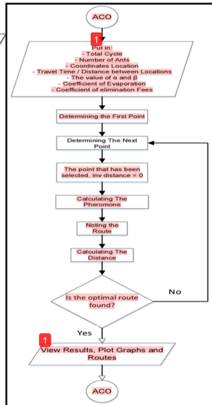
Figure 2. ACO Algorithm used in MATLAB
