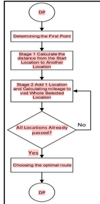
Figure 7. Dynamic programming algorithm
