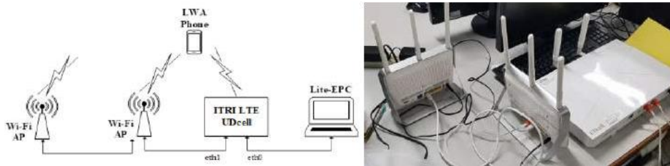
Figure 7. Hardware configuration scheme for two Wi-Fi APs
