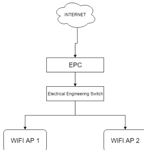
Figure 9. Hardware configuration for two Wi-Fi APs using switch
