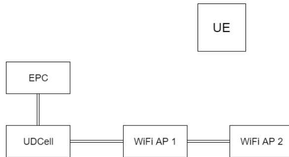
Figure 3. LWA with multiple Wi-Fi APs system
