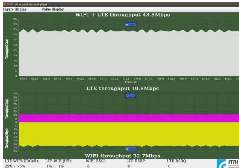
Figure 12. LWA throughput
