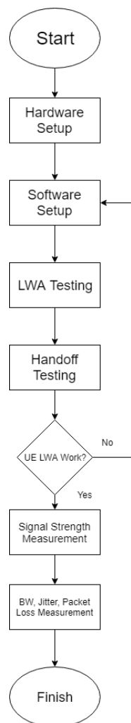
Figure 4. Flowchart of LWA with multiple Wi-Fi APs performance measurement
