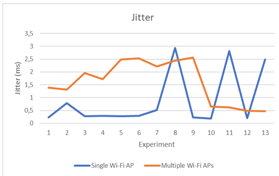
Figure 19. Jitter for single Wi-Fi AP and two Wi-Fi APs comparison
