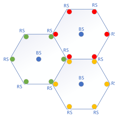
Figure 1. HetNet topology
