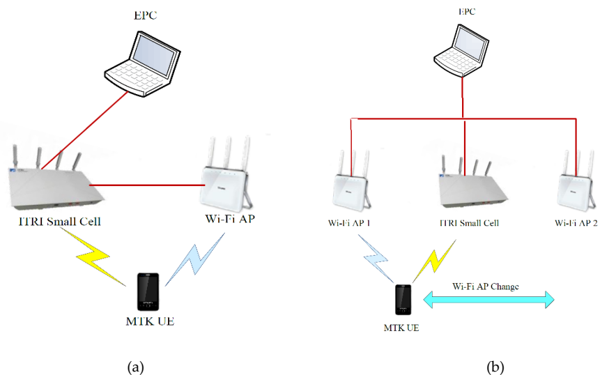
Figure 2. Hardware configuration (a) single Wi-Fi AP (b) multiple Wi-Fi APs
