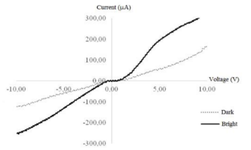
Fig. 1. I-V Curve BST thin film in Dark and Bright condition.
