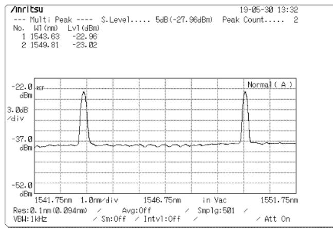
Figure 4. Reflected spectra ( \lambda_1, \lambda_3 ) used for user 1.
