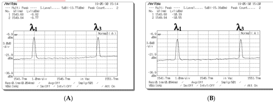
Figure 5. Output spectrum acquired at the output ports of the two electro-optical modulators (EOMs) for different data bits. (A) Optical spectra of EOM 1 for a data bit of “1”. (B) Optical spectra of EOM 2 for a data bit of “0”.
