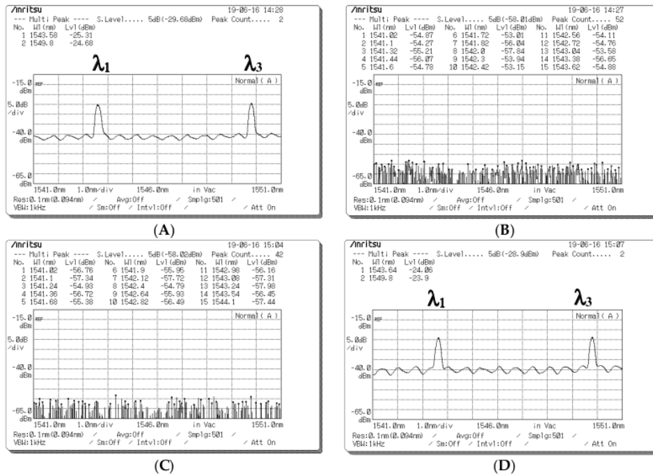
Figure 7. Optical spectrum acquired at the output ports of the polarization beam splitter (PBS) in Decoder 1 when different data bits (D) are sent from Encoder 1. Depolarized spectra acquired at (A) Output Port 1 and (B) Output Port 2 of the PBS when a data bit of “1” is sent. Depolarized spectra acquired at (C) Output Port 1 and (D) Output Port 2 of the PBS when a data bit of “0” is sent.
