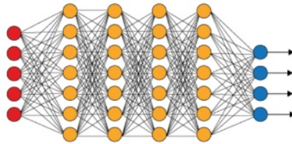
Figure 3: Deep learning
