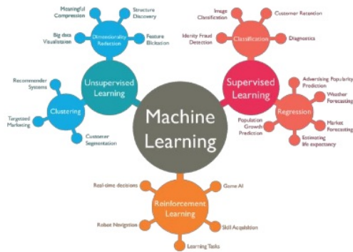
Figure 2: Machine learning
