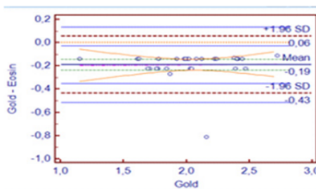
Figure 2. Reliability coefficient of Bland Altman test result. The mean difference of Bland Altman was -0.19.
