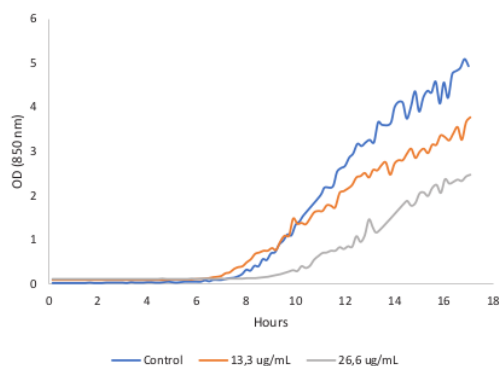
Figure 5. Planktonic Growth Curve of Candida albicans . Note. OD: Optical density.
